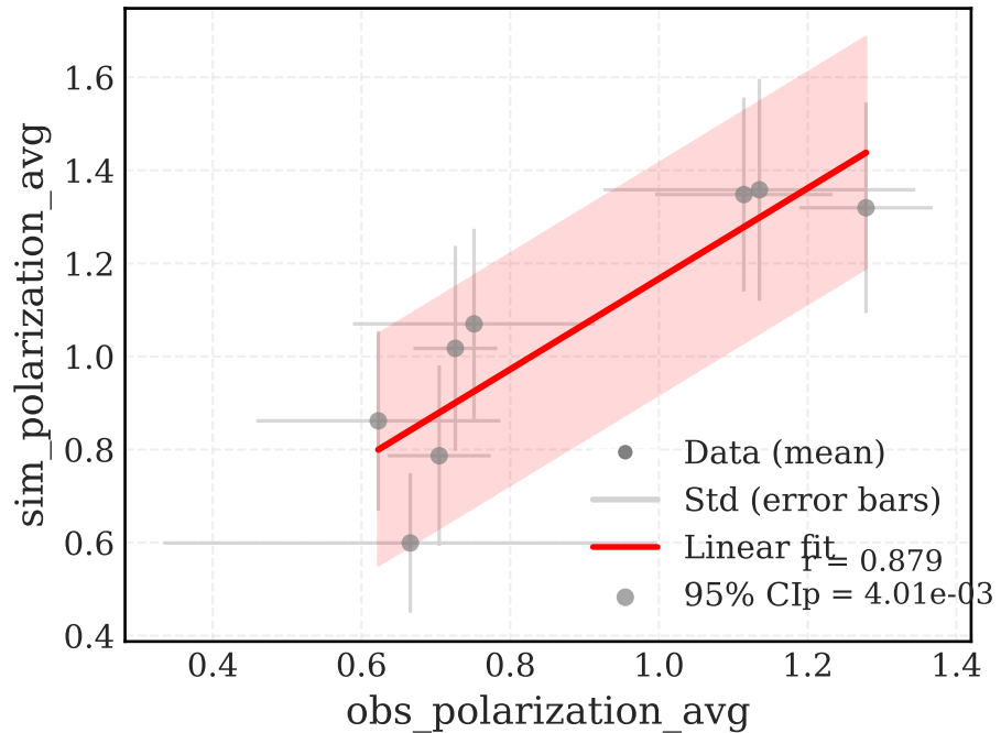
Polarization: Observed vs Simulated
