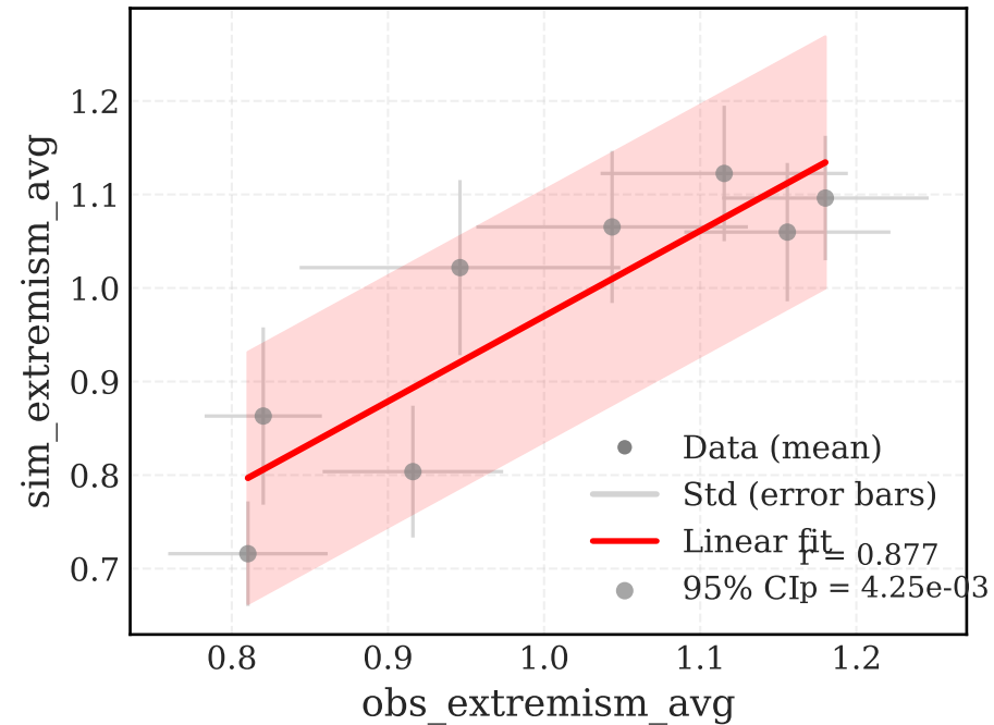
Extremism: Observed vs Simulated
